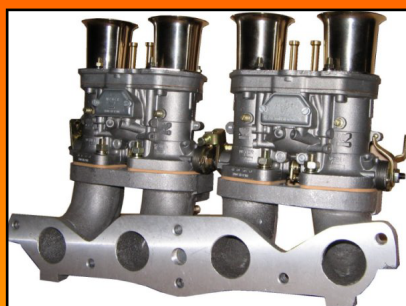
Twin Weber IDF carburettor kit for Ford 2.0 OHC
